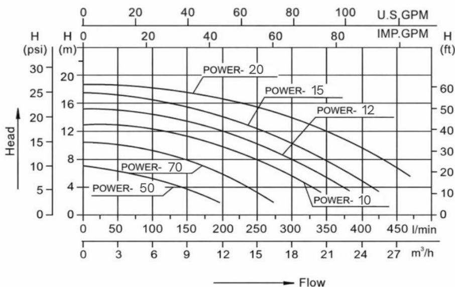
Performance curves
